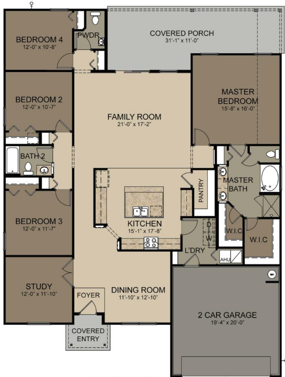
FLOOR PLAN
