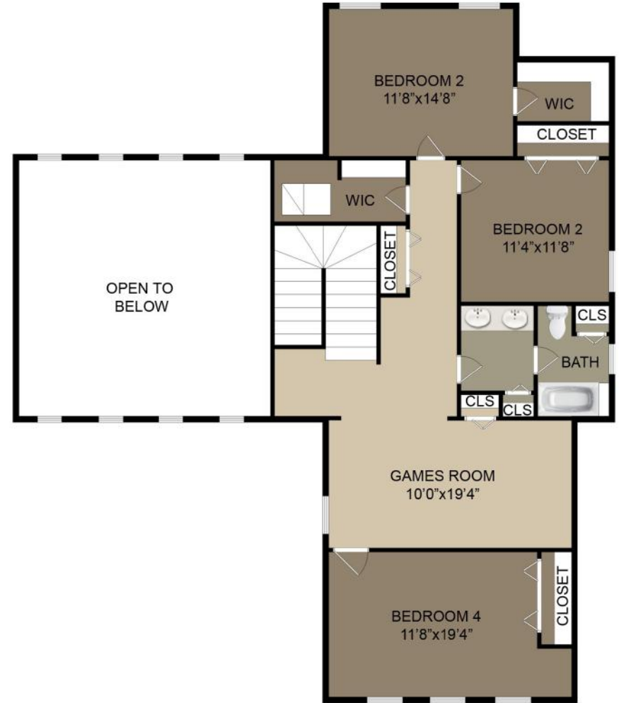
SECOND FLOOR
